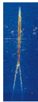
ATOM BEAM IS SPLIT in two by a nanofabricated magnetic wave guide.
